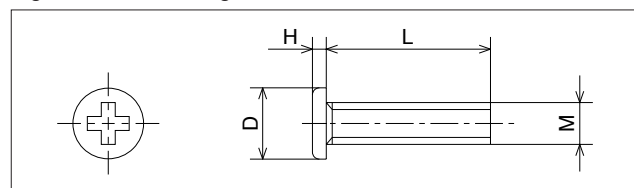
Figure H-34 Mounting Screw
